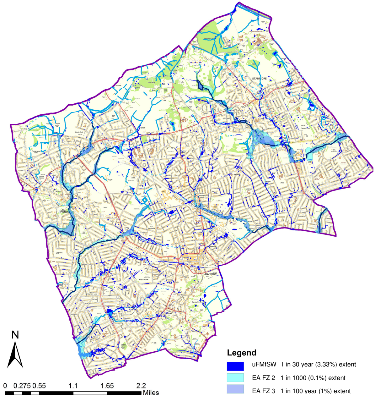
Figure 4.5.2 EA Updated Flood Map for Surface Water (uFMfSW) & Fluvial Flood Zones
